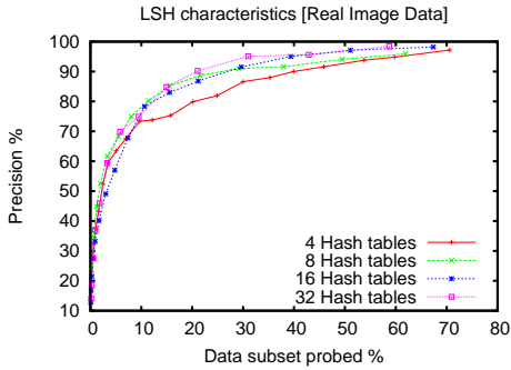
Figure 3: LSH characteristics on picture data.
