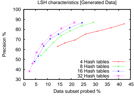
Figure 2: LSH characteristics on generated data.
