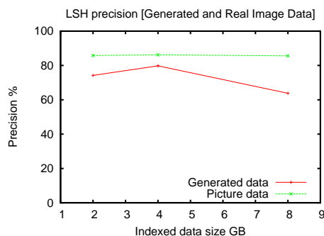
Figure 7: LSH precision on generated and picture data.
