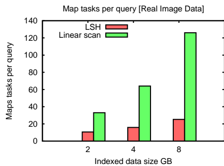
Figure 6: Map tasks per query on picture data.
