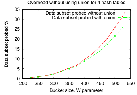
Figure 4: Overhead without using union.
